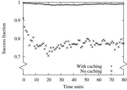
Fig. 3. Success rate with only obedient nodes
