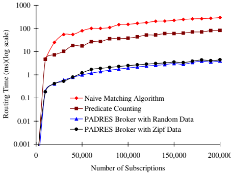
Fig. 12. Publication Matching Time
