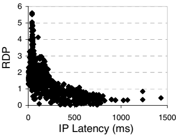
Fig. 23. RDP vs. IP latency using GNP in MEDYM deployment
