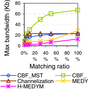
Fig. 16. Maximum server bandwidth consumption in single-publisher case
