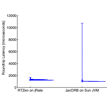
Fig. 7. Consistency: Comparison of RTZen on jRate and JacORB on Sun JVM
