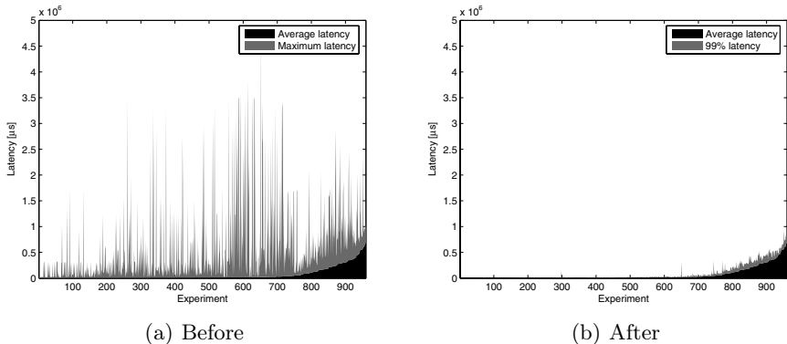
Fig. 3. The “haircut” effect of removing 1% of the outliers
