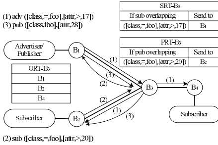
Fig. 1. Broker Network
