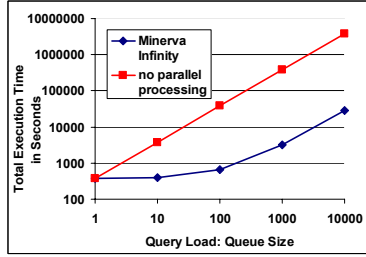
Fig. 3. Scalability Results
