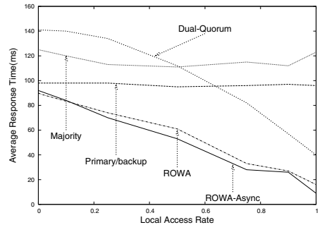
(b) 5% write rate & varying access locality
