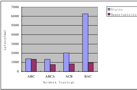
Fig. 15. Average Latency (100% data)
