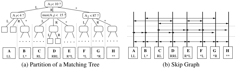
Fig. 3. Peer-to-peer Matching Tree
