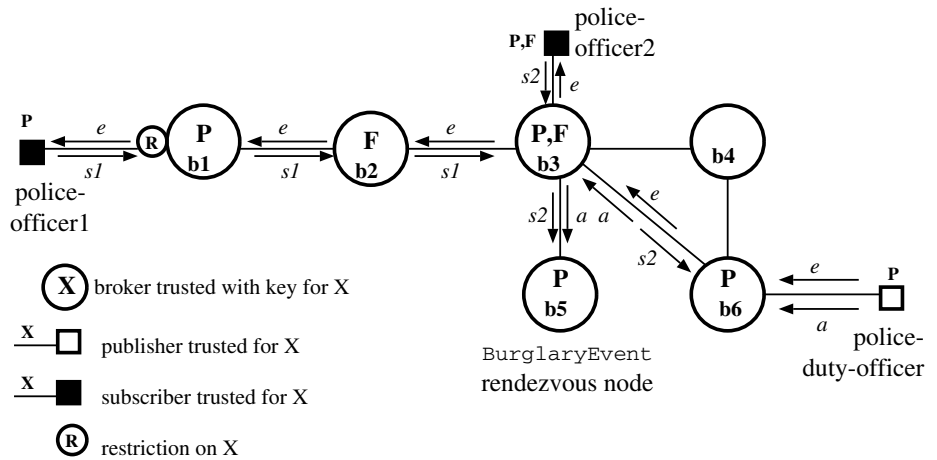
Fig. 4. Notifying two police officers of a BurglaryEvent
