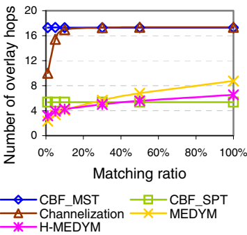
Fig. 20. Average event path length in simulation
