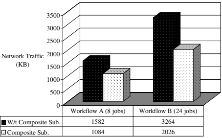
Fig. 15. Workflow Traffic
