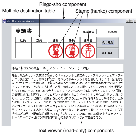
Fig. 6. Ringi-sho compound document
