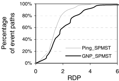
Fig. 22. Cumulative Distribution of RDP in MEDYM deployment
